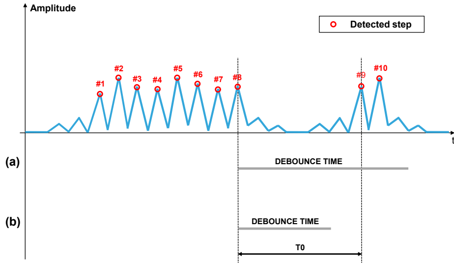
Figure 19. Pedometer debounce
