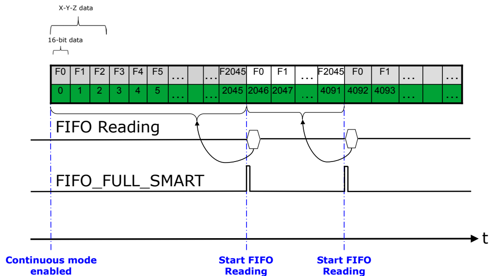
Figure 29. Continuous mode
