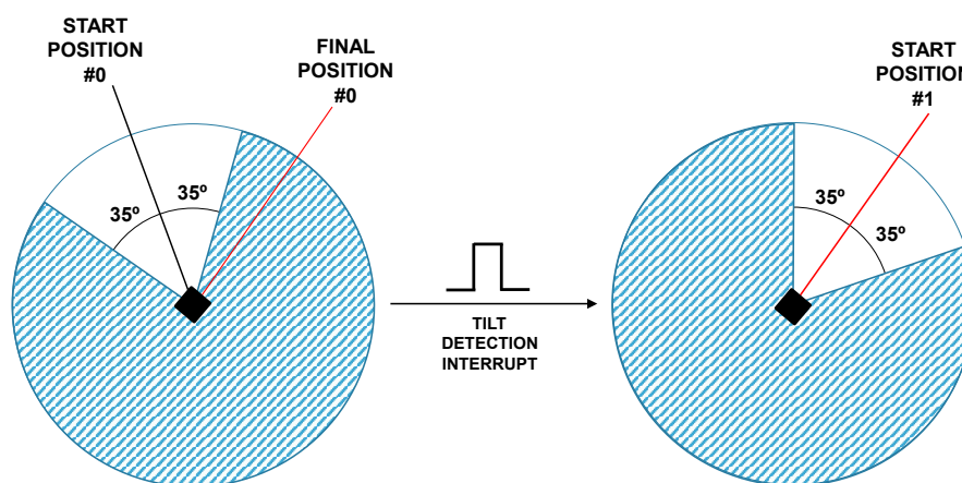
Figure 21. Tilt example
