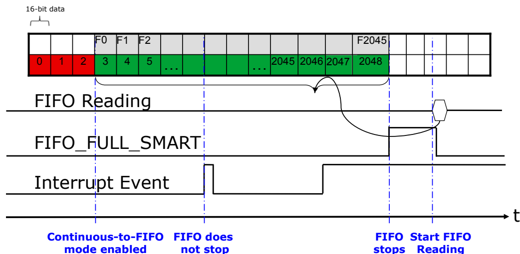
Figure 30. Continuous-to-FIFO mode
