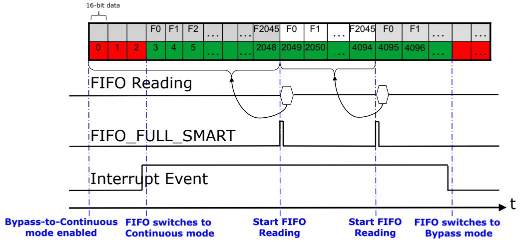
Figure 31. Bypass-to-Continuous mode
