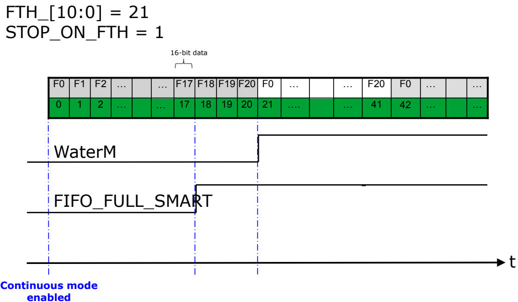
Figure 35. FIFO threshold (STOP_ON_FTH = 1) in Continuous mode
