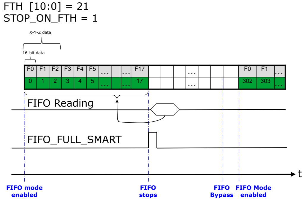
Figure 34. FIFO threshold (STOP_ON_FTH = 1) in FIFO mode
