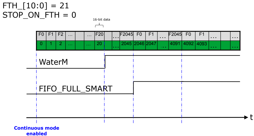
Figure 33. FIFO threshold (STOP_ON_FTH = 0) shows an example of FIFO threshold level usage when just accelerometer (or gyroscope) data are stored. The STOP_ON_FTH bit set to 0 in the FIFO_CTRL4 register. The threshold level is set to 21 through the FTH_[10:0] bits. The WaterM bit of the FIFO_STATUS2 register rises after the 21 st level has been reached (21 samples in the FIFO). Since the STOP_ON_FTH bit is set to 0, the FIFO will not stop at the 21 st sample, but will keep storing data until the FIFO_FULL_SMART flag is set high.
