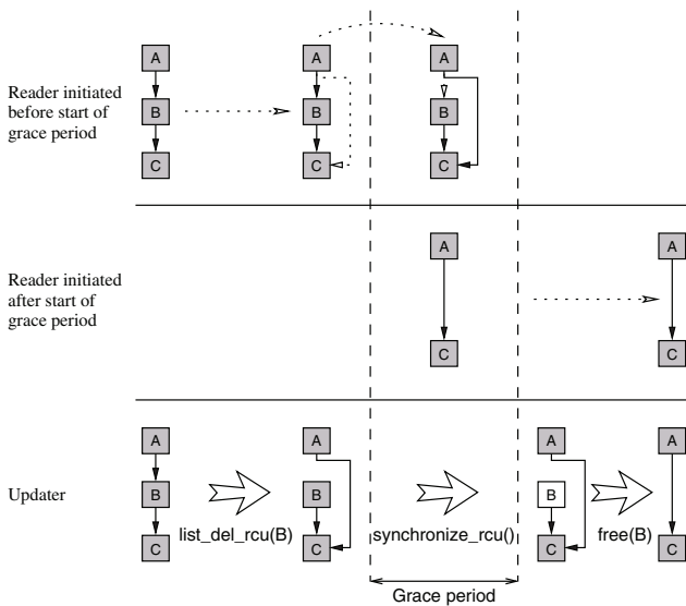
Fig. 3. RCU linked-list deletion.
