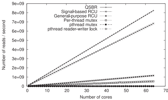
Fig. 4. Read-side scalability of various synchronization primitives, 64-core POWER5+.
