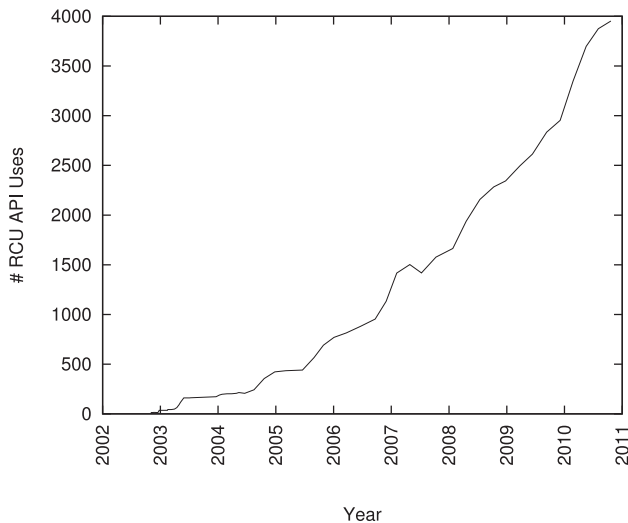
Fig. 1. Linux-Kernel usage of RCU.
