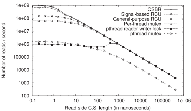
Fig. 7. Impact of read-side critical section length, eight reader threads on 64-core POWER5+, logarithmic scale.
