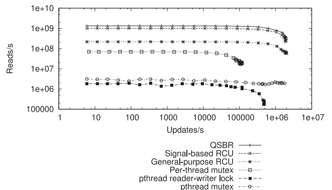
Fig. 9. Update overhead, 8-core Intel Xeon, logarithmic scale.
