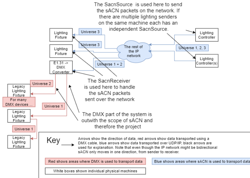
Figure 13: A diagram showing where the 2 separate parts of the project are expected to be utilised within an sACN and DMX system
