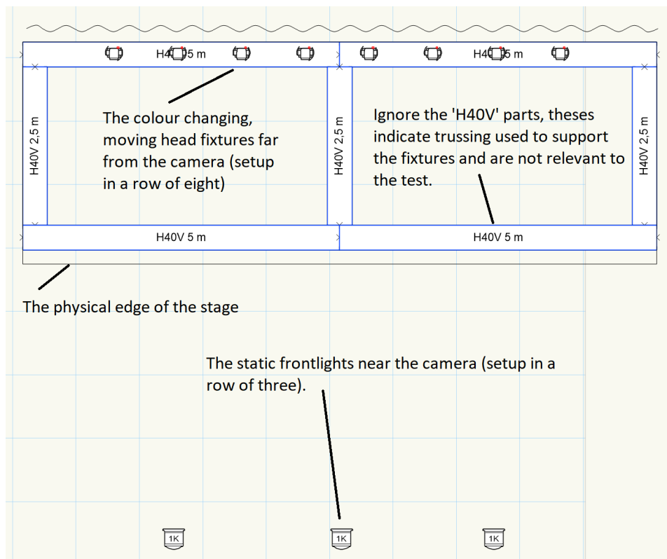
Figure 27: The lighting plot showing the locations and addresses of fixtures within the visualiser used as part of the acceptance test. This is based on the actual lighting layout used within the students association. Additional explanation has been added on top of the plan to describe what each part means.
