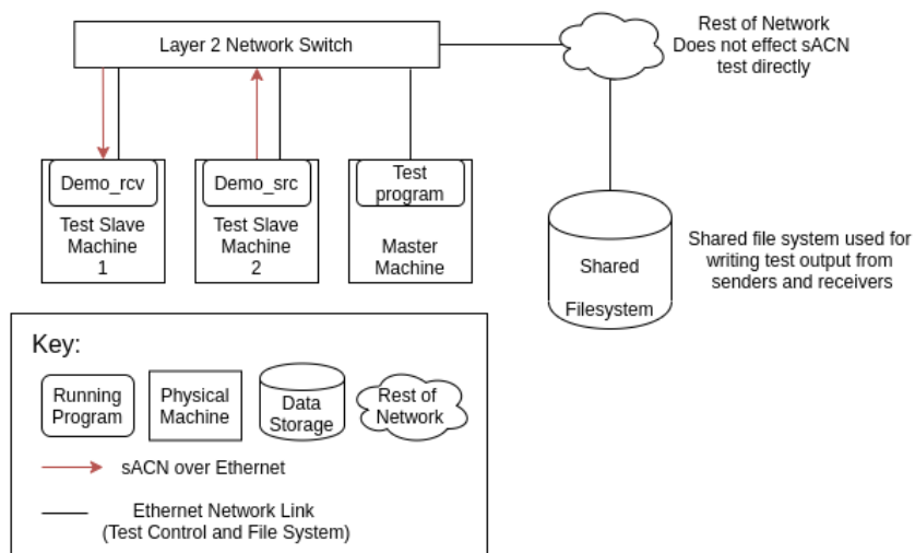
Figure 16: The abstract setup of the integration tests along with the actual implementation
