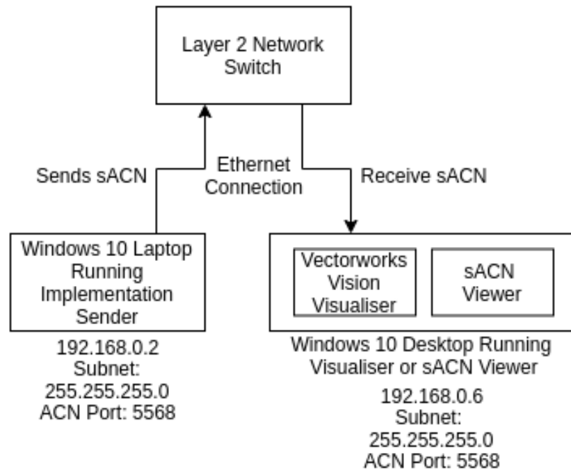
Figure 24: The set-up of the sender implementation interoperability test
