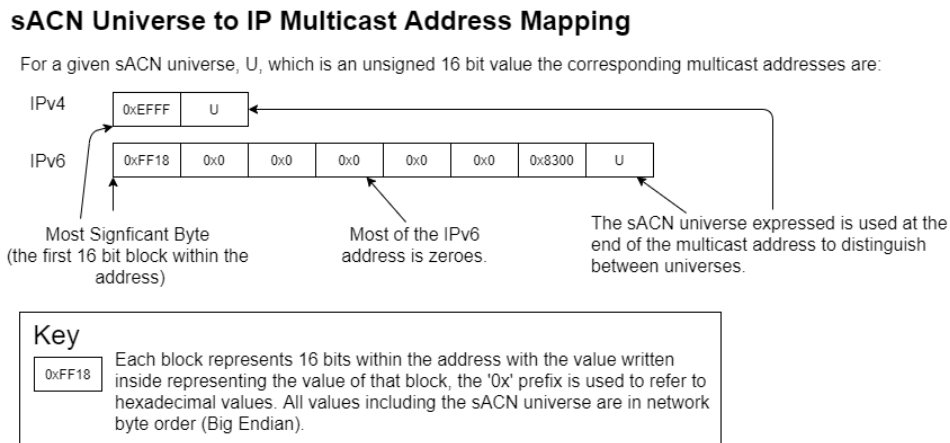
Figure 5: The mapping used from an sACN universe to an IPv4 or IPv6 multicast address within an sACN network
