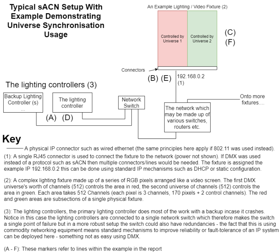
Figure 3: A diagram demonstrating how sACN universe synchronisation allows simultaneous control of multiple DMX universes and its use cases
