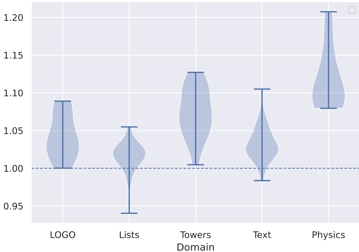
Rewritten corpus size ratio (DreamCoder / Stitch)
